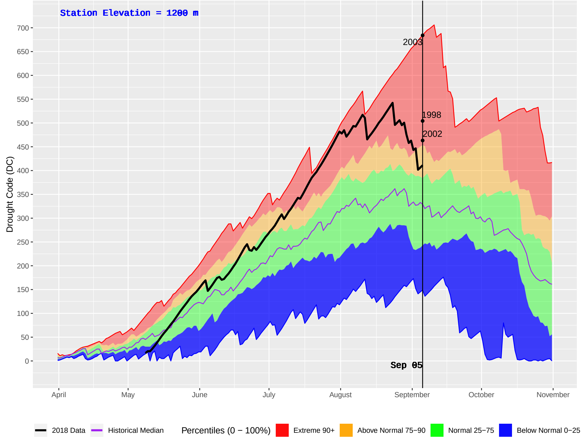
TSAR CREEK (361) : Historical (1986–2016) and Current (2018) Daily Drought Code (DC)
